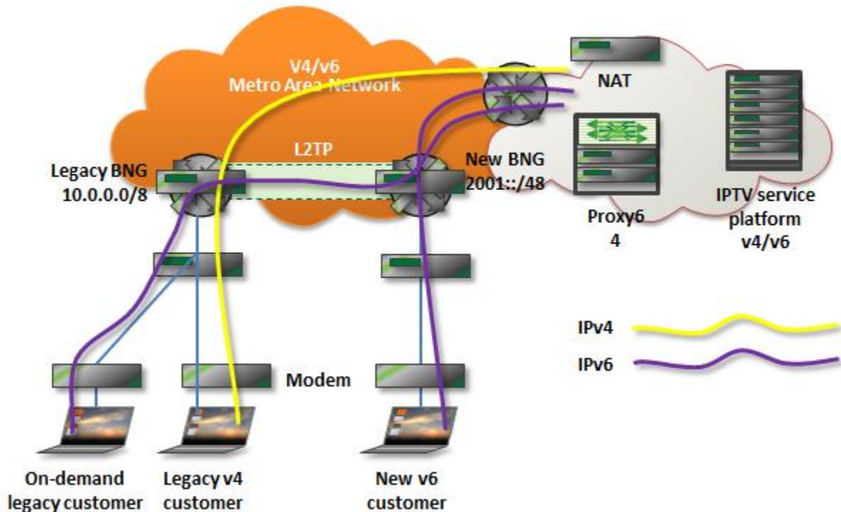
Figure 4 –Network Architecture of SP4
