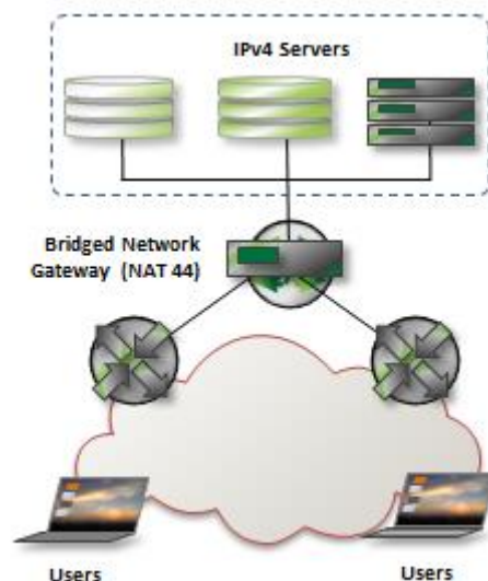
Figure 3 –Network Architecture of SP3
